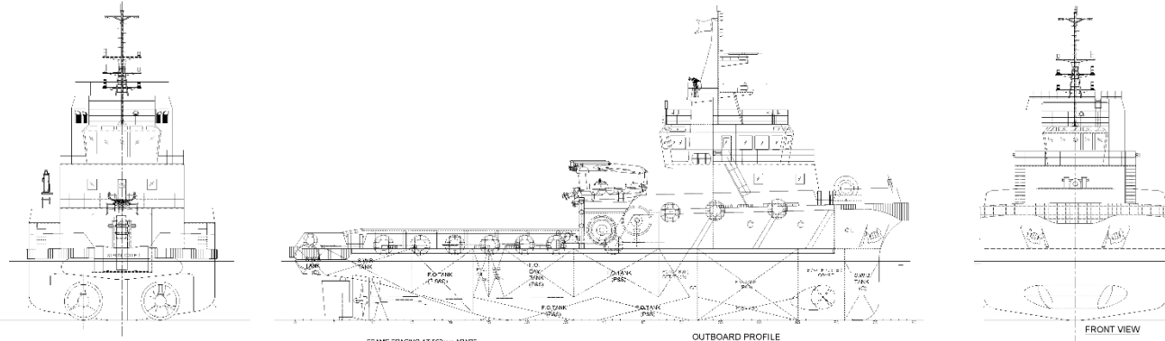
STERN VIEW
